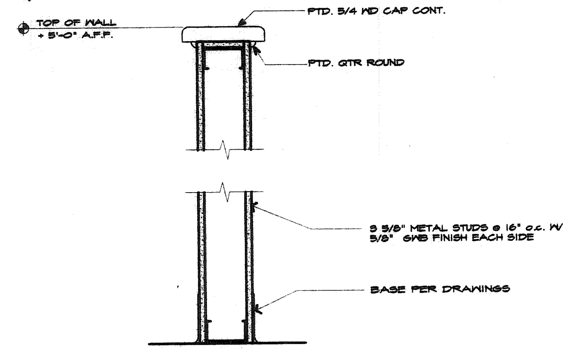
2 WALLTYPE 2 - TYPICAL KNEE WALL CONSTRUCTION
