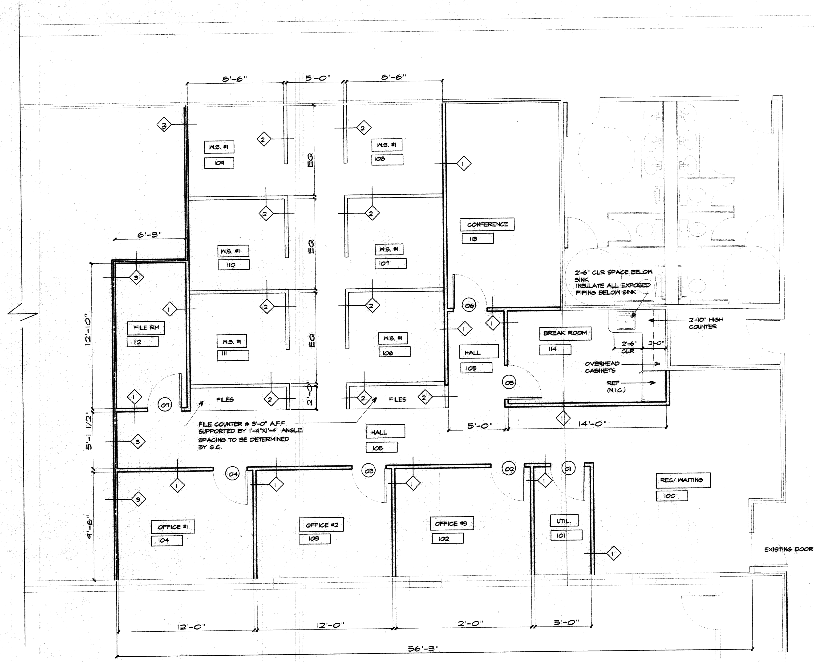
1 FIRST FLOOR PLAN SCALE: 1/4" = 1'-0"
