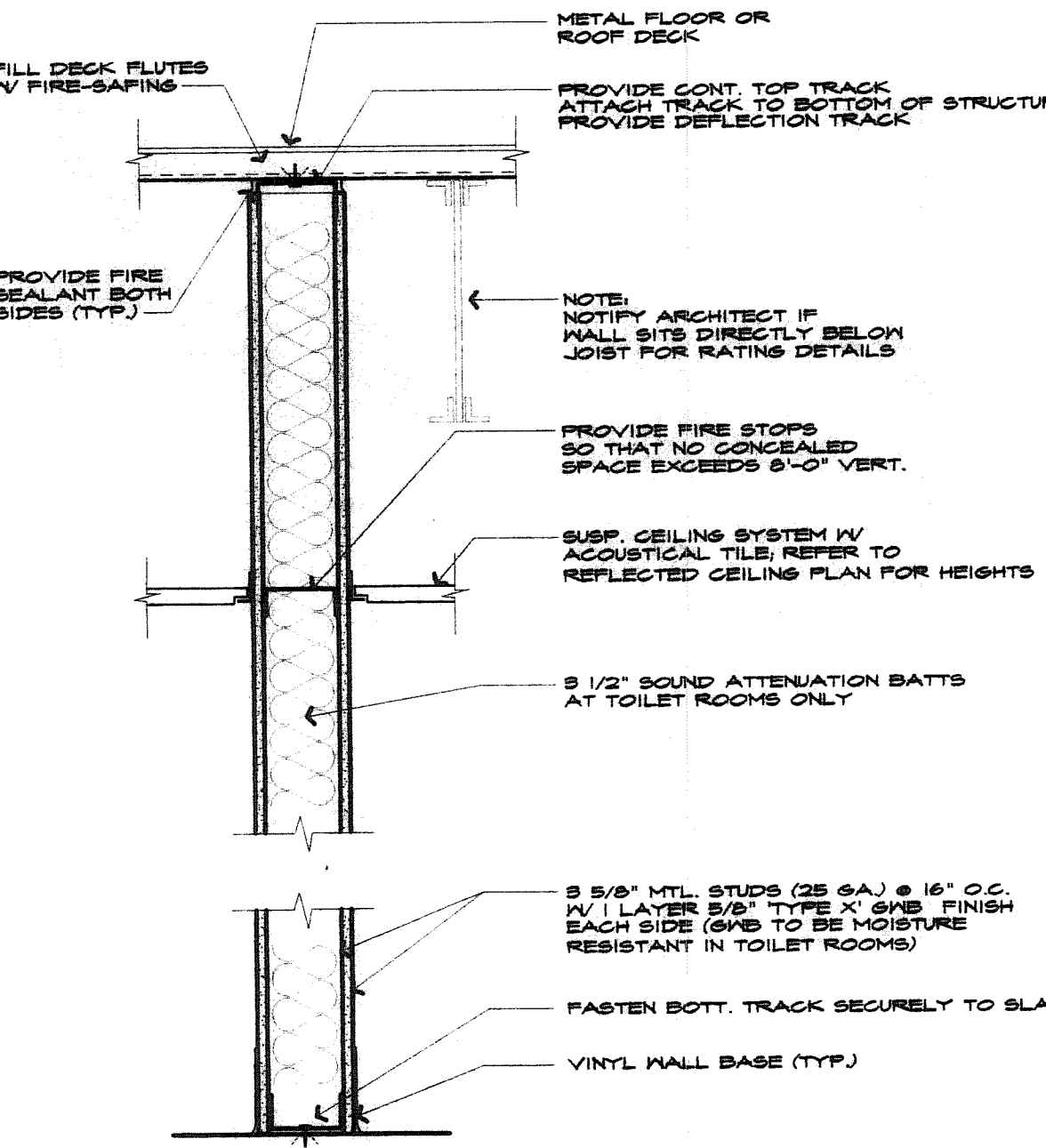
3 WALLTYPE 3 - TYPICAL ONE HOUR RATED WALL WITH 3 5/8" METAL STUDS
