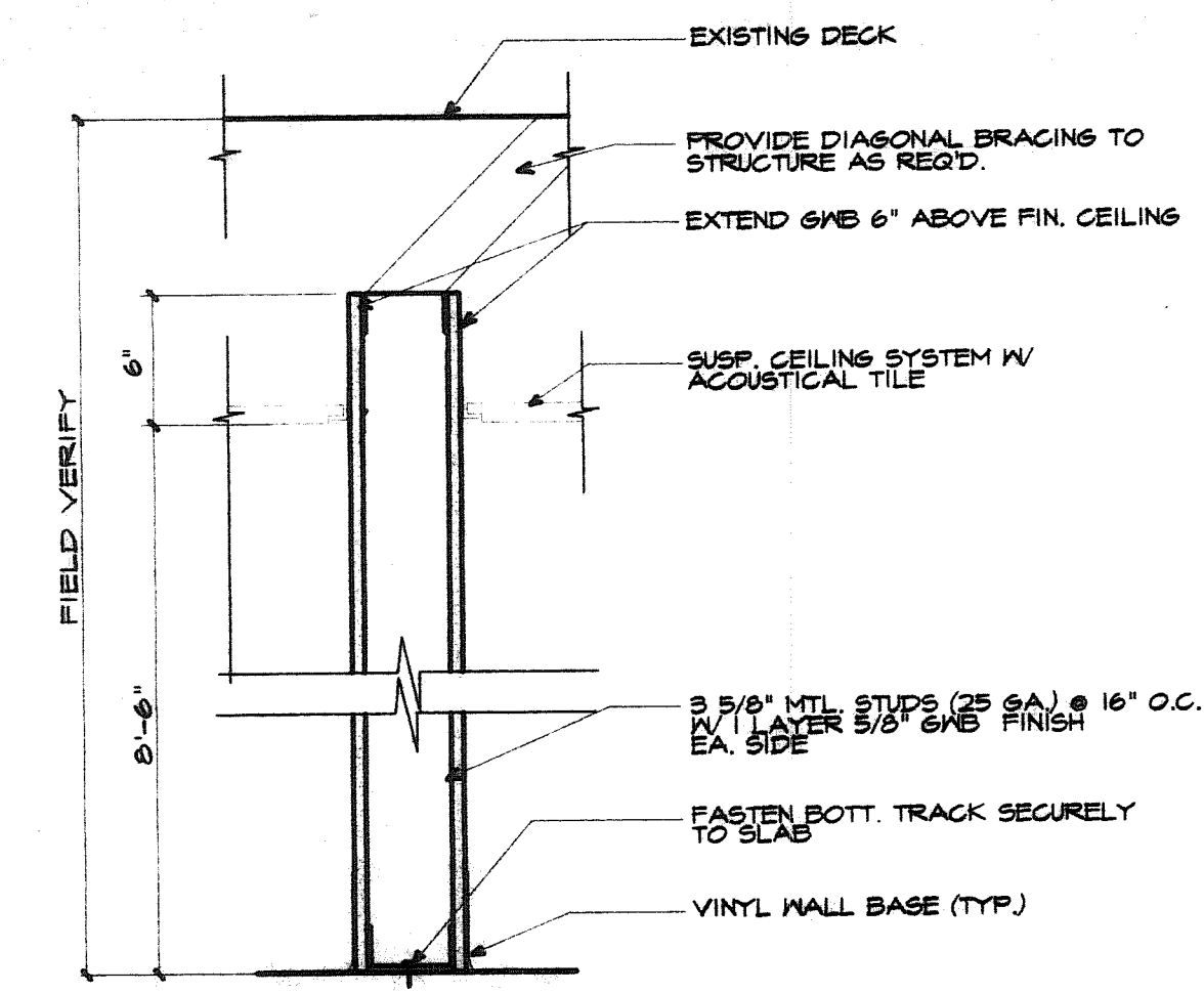
1 WALLTYPE 1 - TYPICAL NON-RATED PARTITION WITH 3 5/8" METAL STUDS
